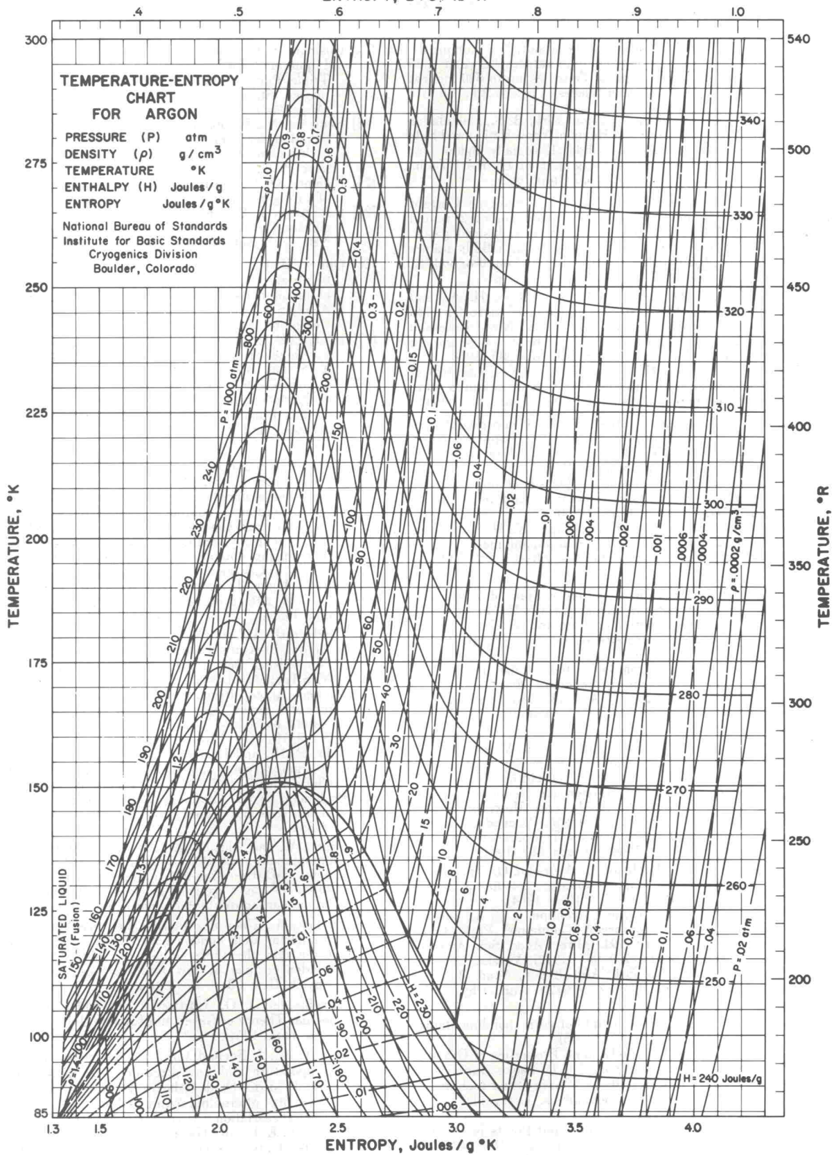
FIGURE 24. Temperature-entropy chart.
